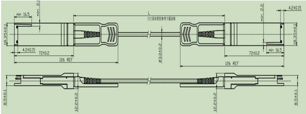
Figure 4, Mechanical Design Diagram
