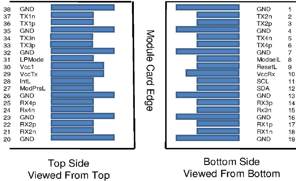
Figure 2, Pin View
